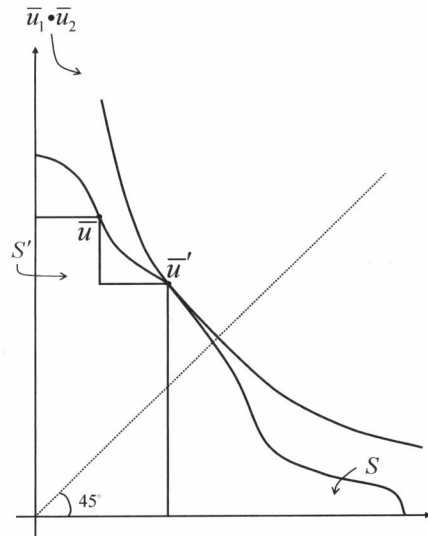
図6 \bar{\mathbf{u}} \in F(S) \cap F(S') by CI
