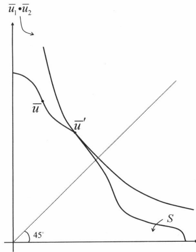
図6 \bar{\mathbf{u}} \in F(S) \cap F(S') by CI
